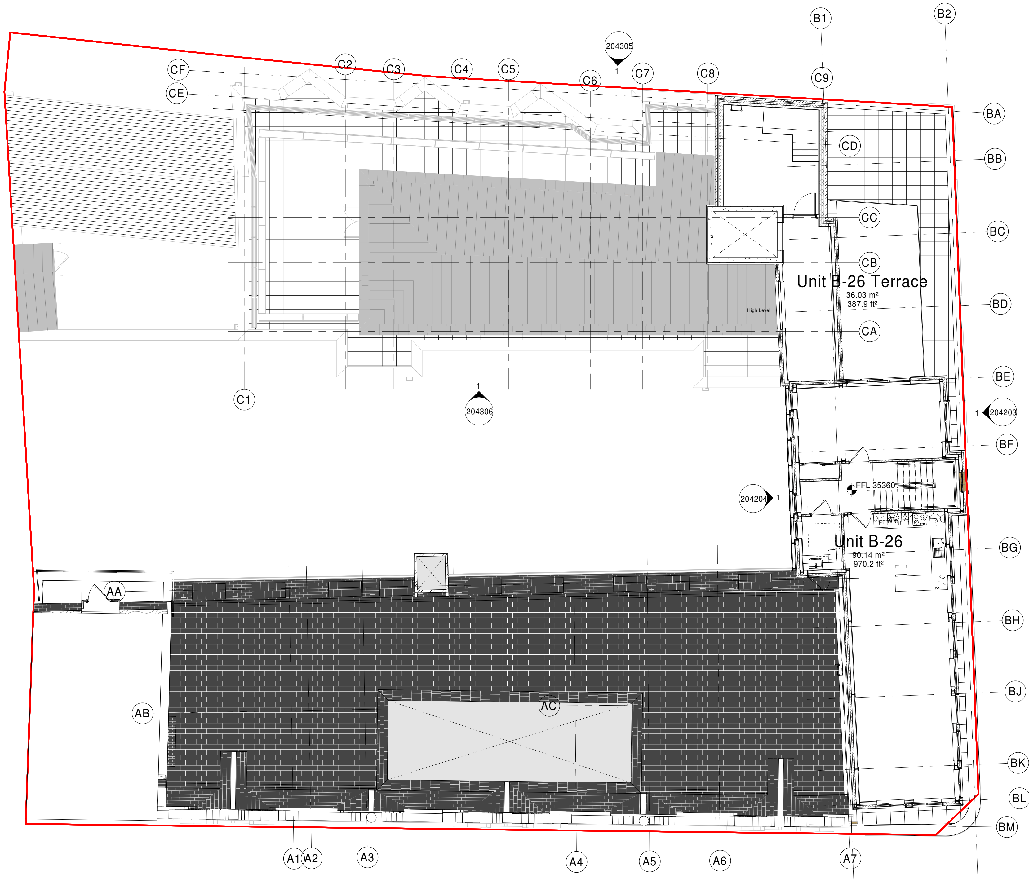
Level 4-All Blocks-GA Planning 1 : 100
